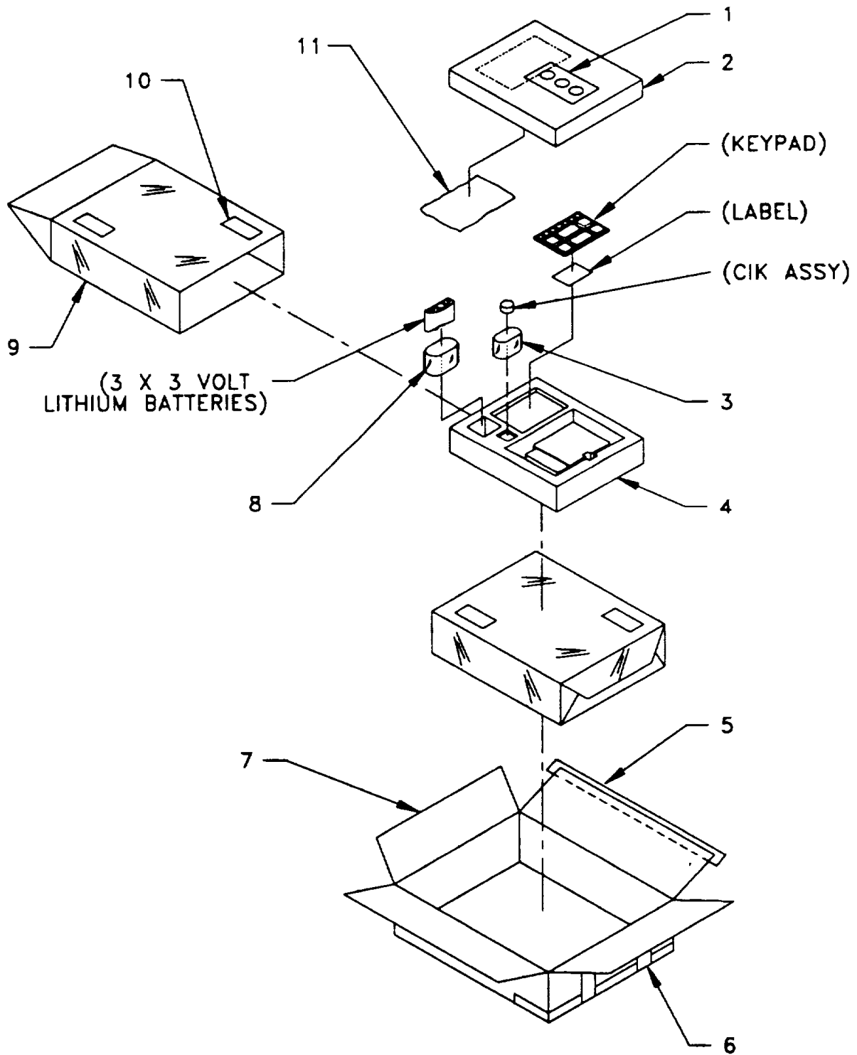
Figure 2-4. ANCD Packaging
