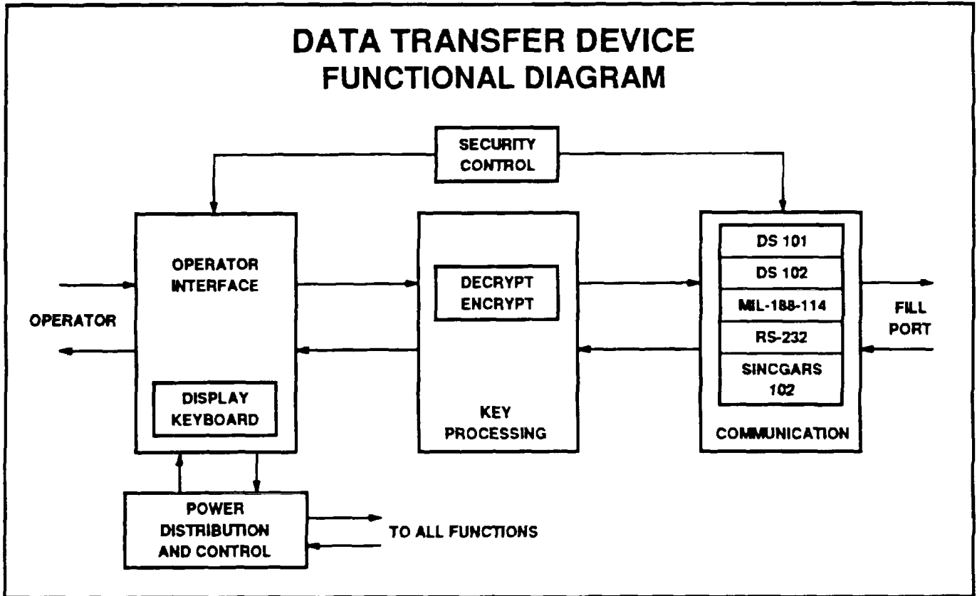
Figure 1-3. ANCD Subsystem, Simplified Block Diagram
