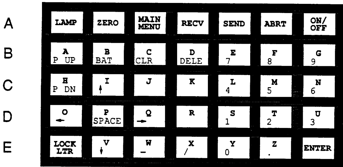
Figure 2-2. ANCD Keys
