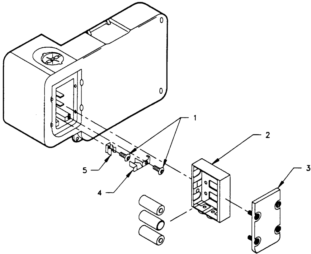
Figure 3-1. Battery Replacement
