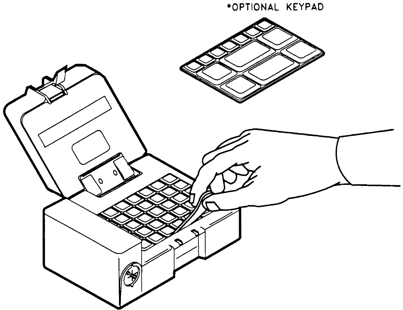
Figure 4-3. Keypad Removal Replacement
